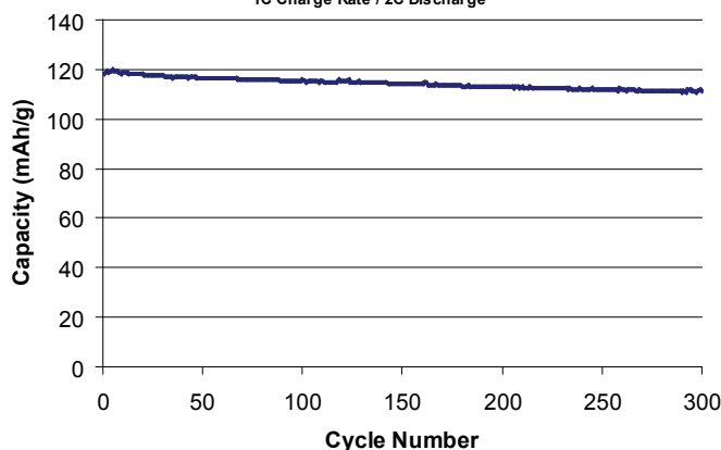
Cycling Performance at 23°C 1C Charge Rate / 2C Discharge
